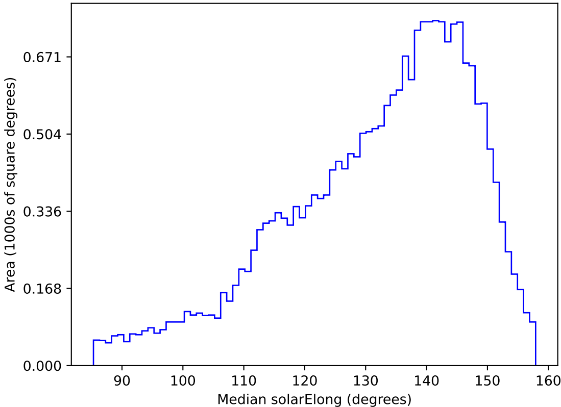
too_elab_r32_d3_gz_v3.4_10yrs All sky u band: Median solarElong
