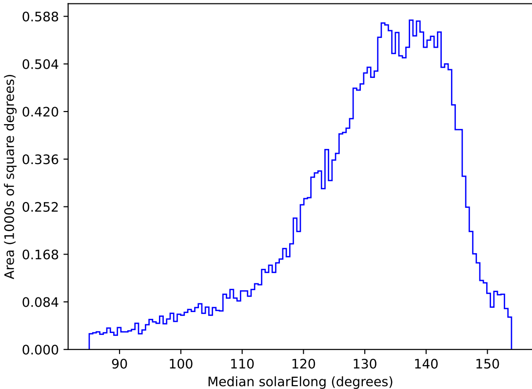
too_elab_r32_d3_gz_v3.4_10yrs All sky r band: Median solarElong
