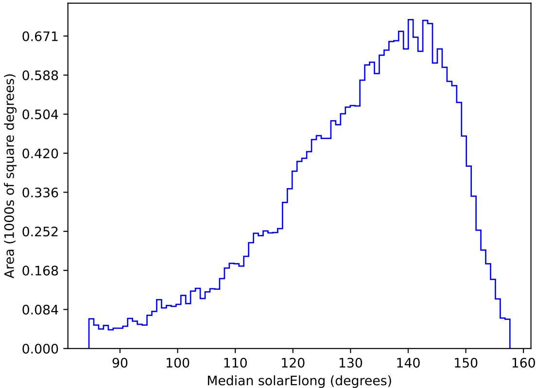
too_elab_r32_d3_gz_v3.4_10yrs All sky g band: Median solarElong
