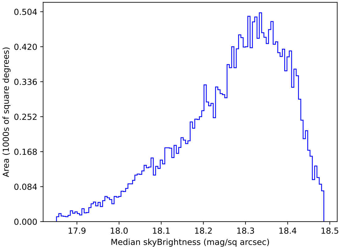
too_elab_r32_d3_gz_v3.4_10yrs Yr 1 y band: Median skyBrightness
