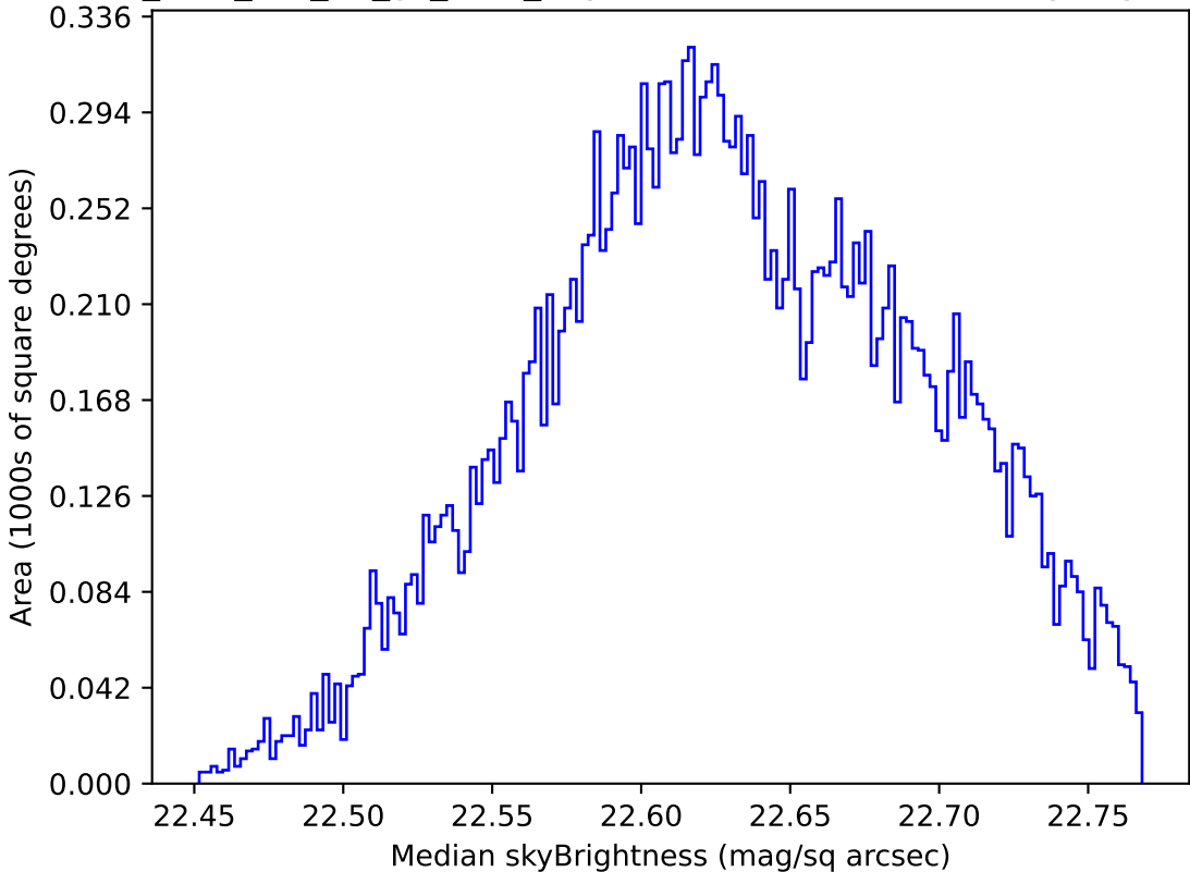
too_elab_r32_d3_gz_v3.4_10yrs Yr 1 u band: Median skyBrightness
