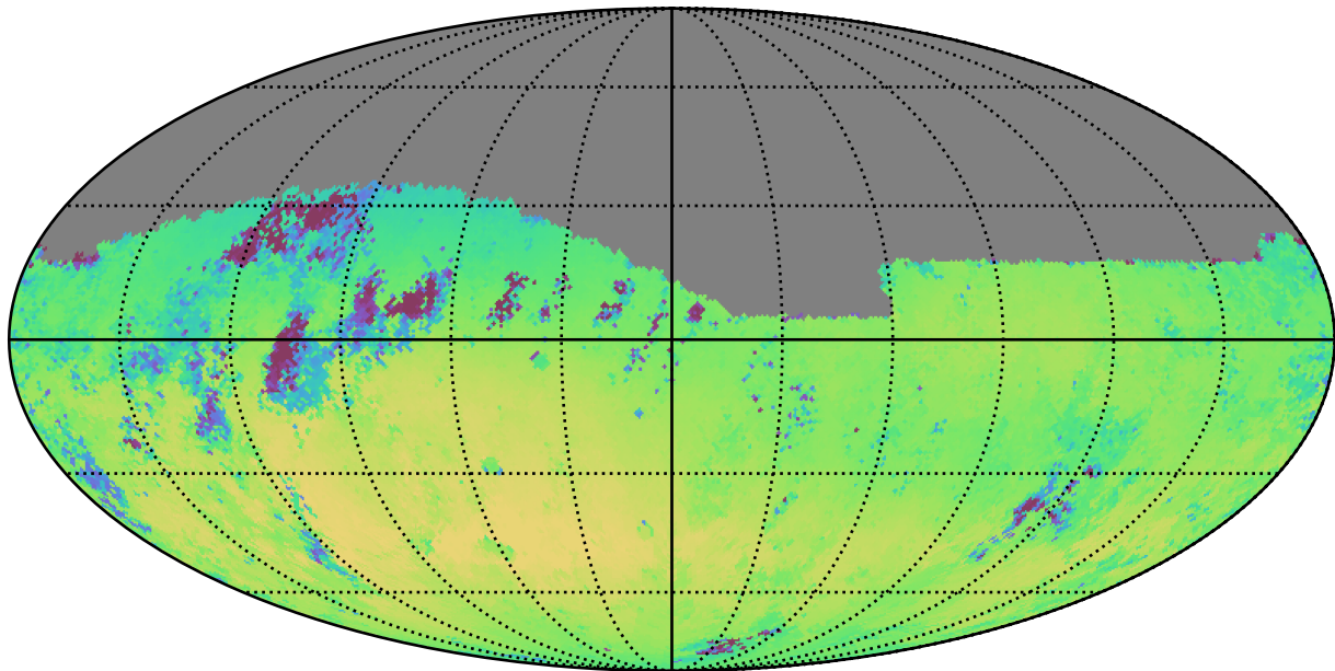
too_elab_r32_d3_gz_v3.4_10yrs Yr 1 r band: Median skyBrightness
