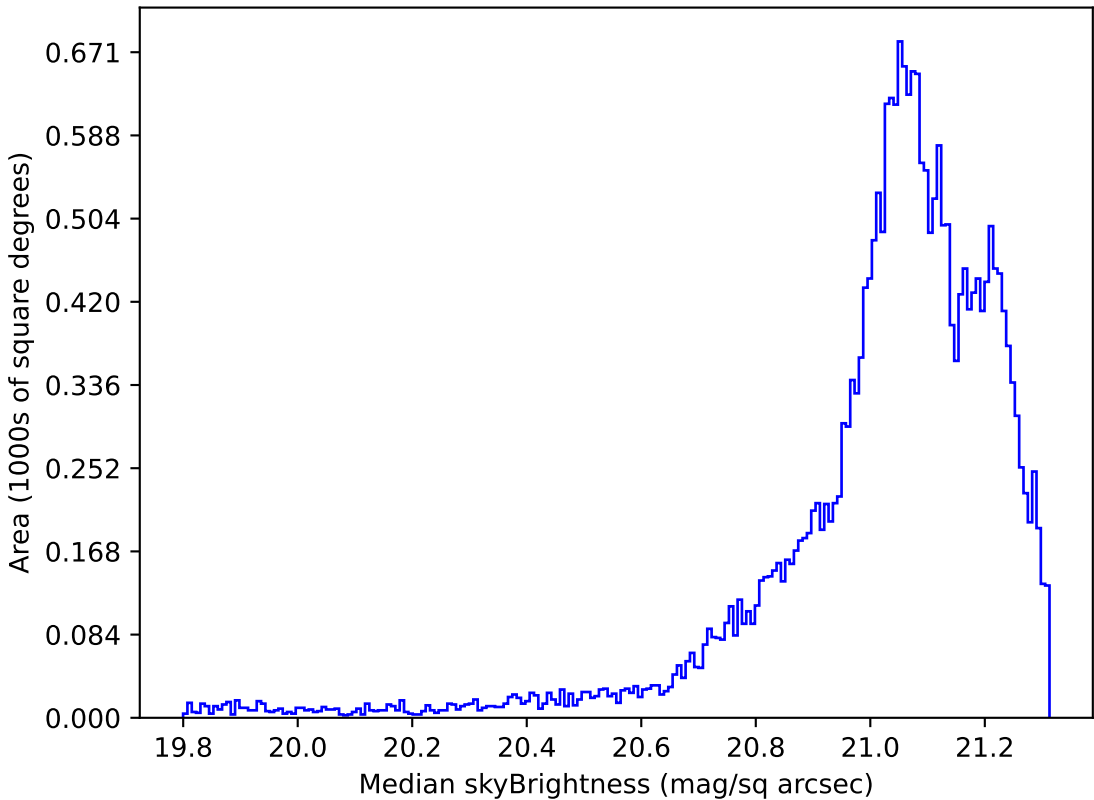
too_elab_r32_d3_gz_v3.4_10yrs Yr 1 r band: Median skyBrightness
