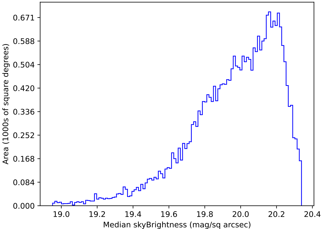
too_elab_r32_d3_gz_v3.4_10yrs Yr 1 i band: Median skyBrightness
