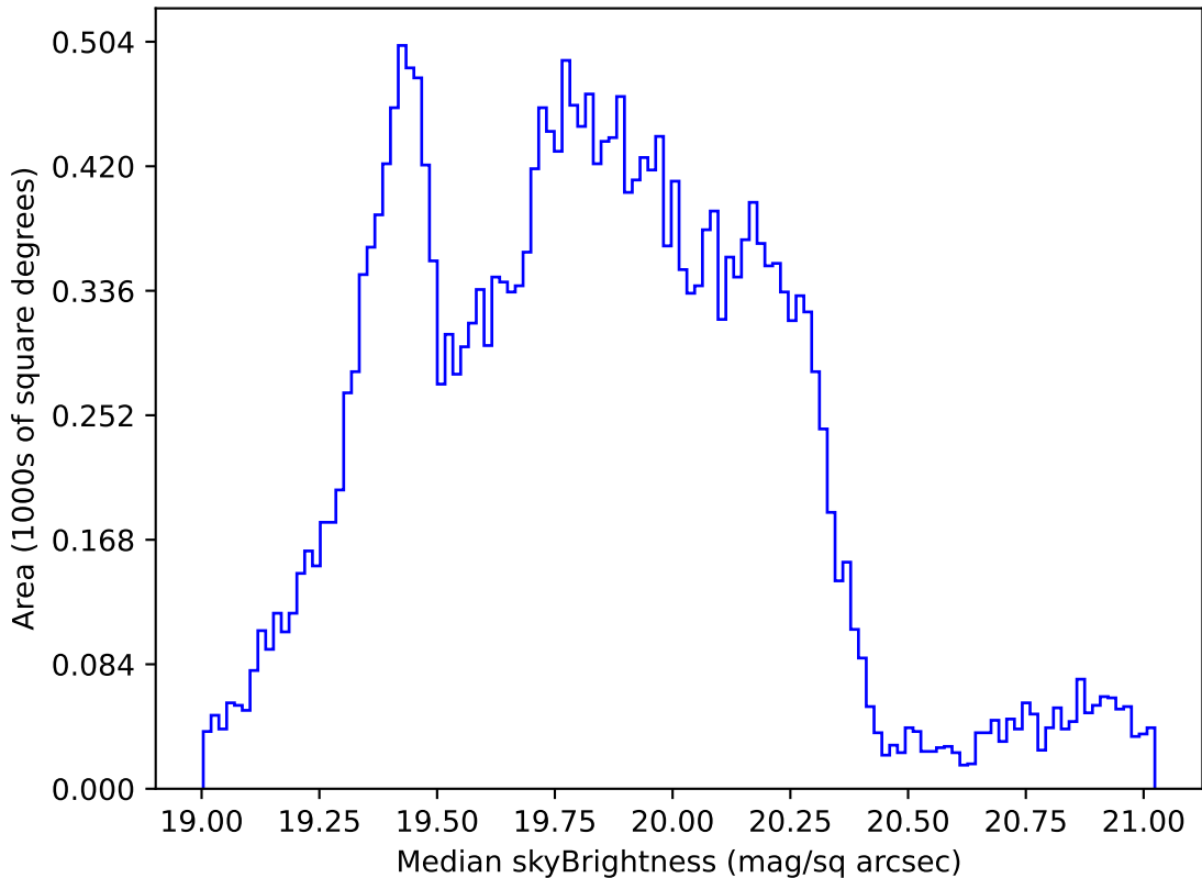
too_elab_r32_d3_gz_v3.4_10yrs Yr 1 all bands: Median skyBrightness
