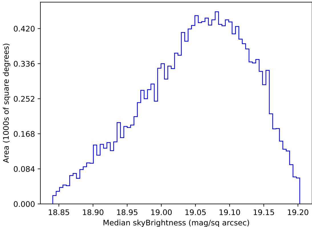
too_elab_r32_d3_gz_v3.4_10yrs WFD z band: Median skyBrightness
