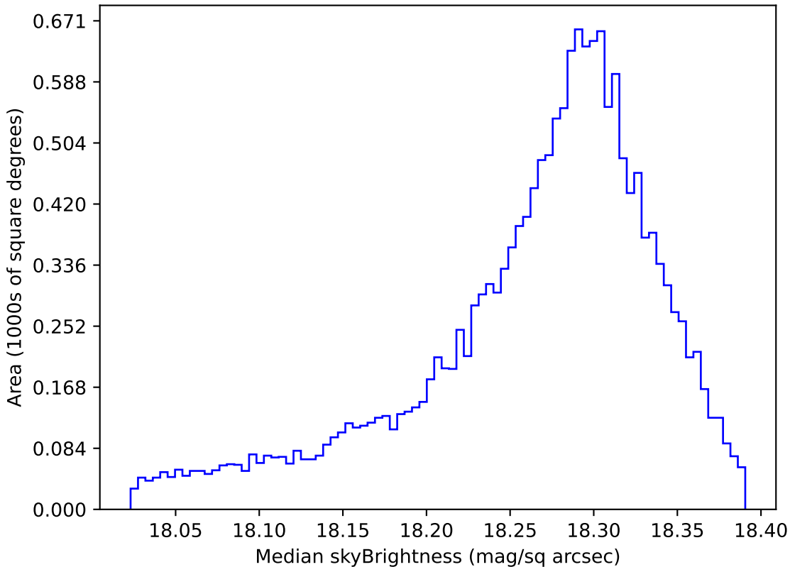
too_elab_r32_d3_gz_v3.4_10yrs WFD y band: Median skyBrightness
