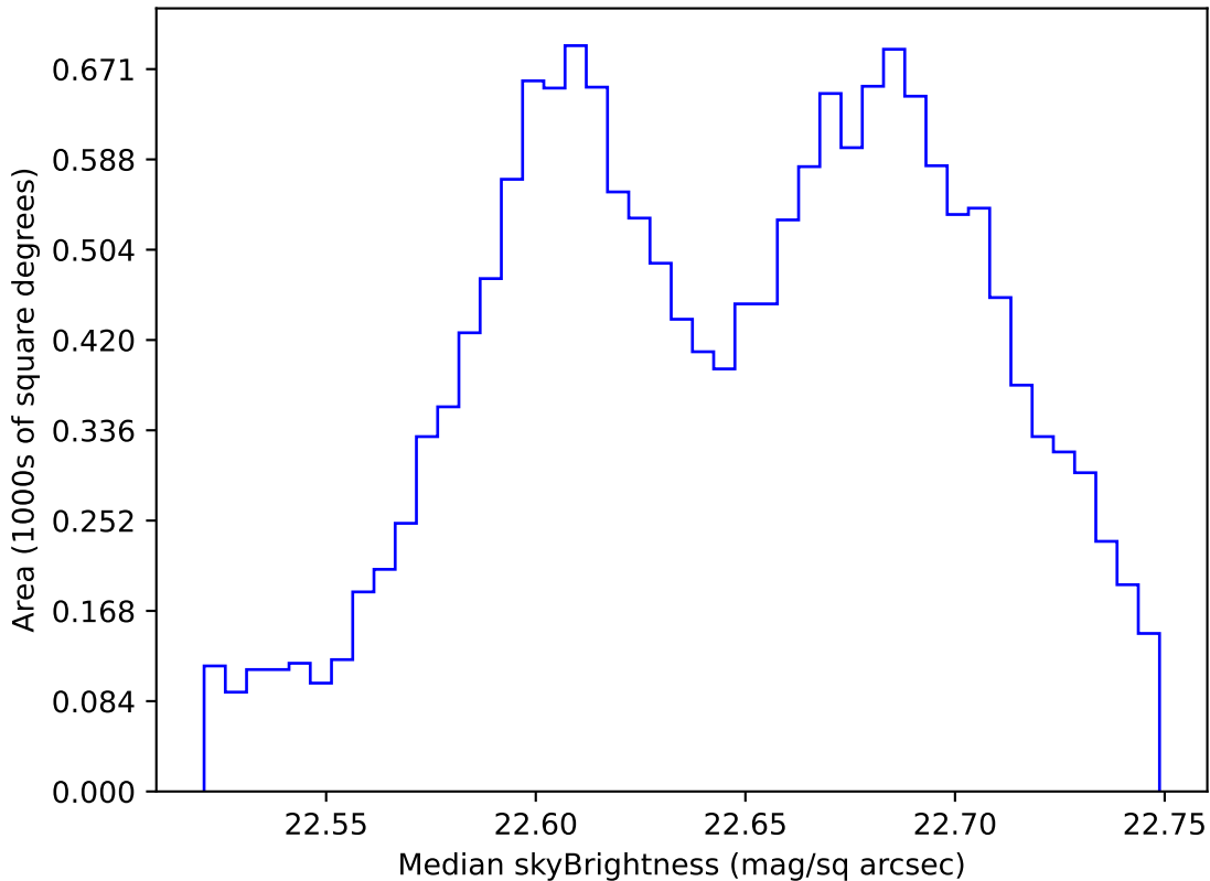
too_elab_r32_d3_gz_v3.4_10yrs WFD u band: Median skyBrightness
