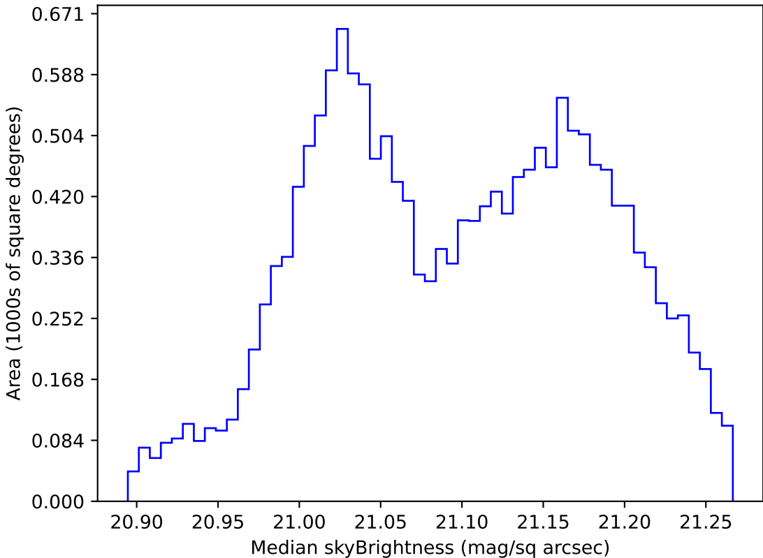
too_elab_r32_d3_gz_v3.4_10yrs WFD r band: Median skyBrightness
