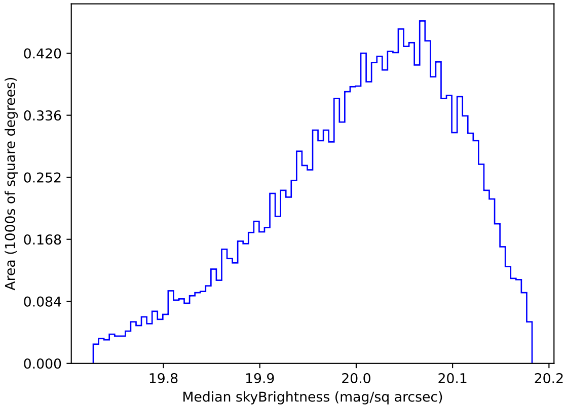
too_elab_r32_d3_gz_v3.4_10yrs WFD i band: Median skyBrightness
