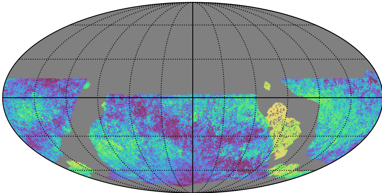
too_elab_r32_d3_gz_v3.4_10yrs WFD all bands: Median skyBrightness
