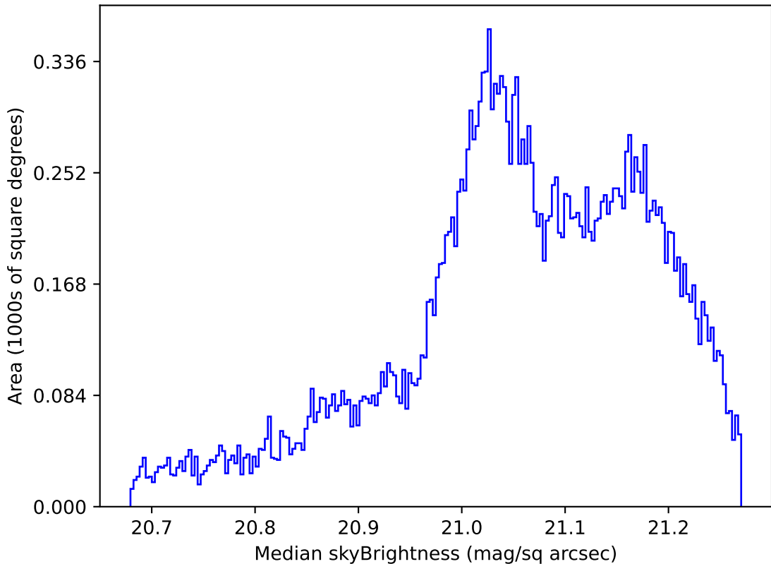
too_elab_r32_d3_gz_v3.4_10yrs All sky r band: Median skyBrightness
