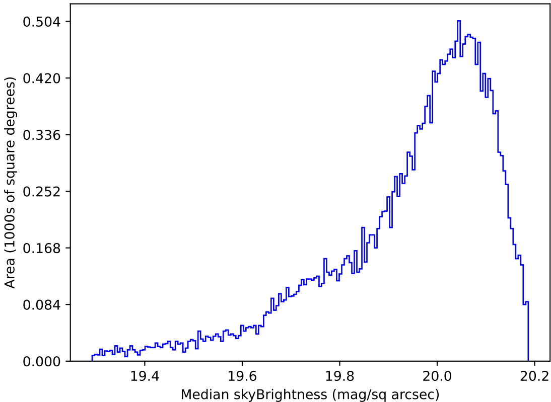
too_elab_r32_d3_gz_v3.4_10yrs All sky i band: Median skyBrightness
