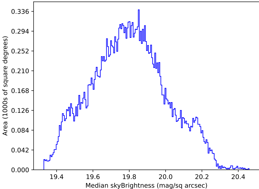
too_elab_r32_d3_gz_v3.4_10yrs All sky all bands: Median skyBrightness
