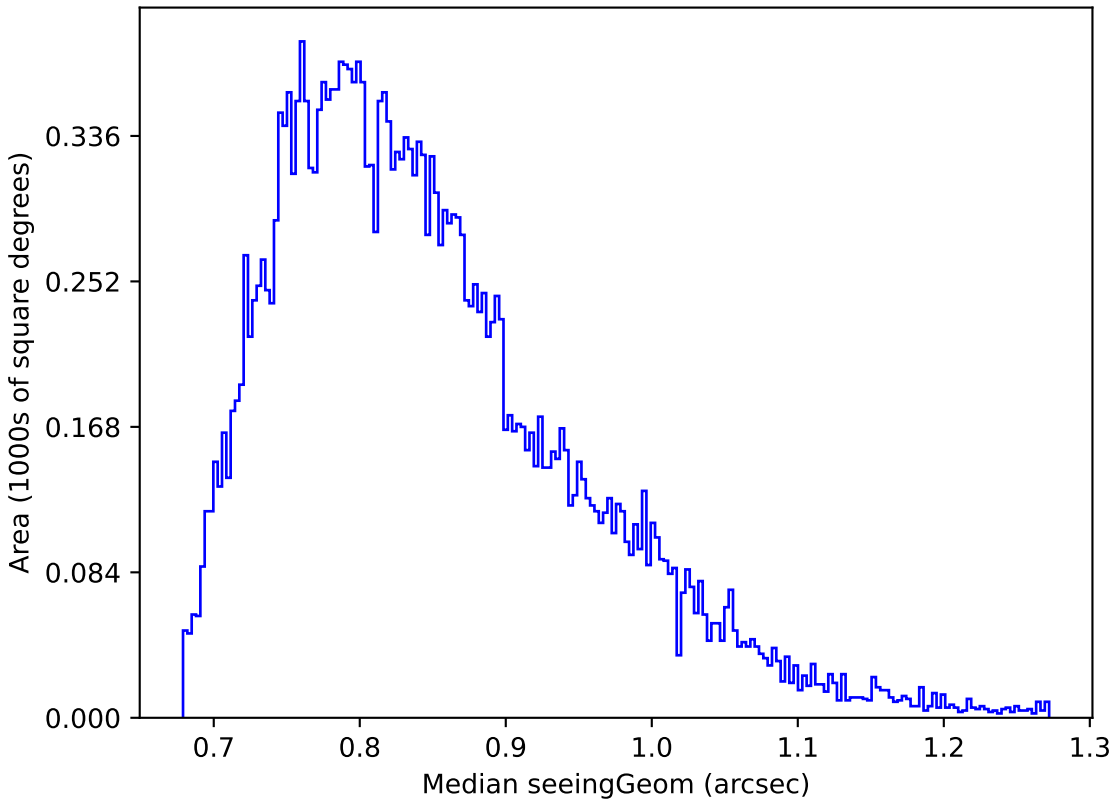
too_elab_r32_d3_gz_v3.4_10yrs Yr 1 z band: Median seeingGeom
