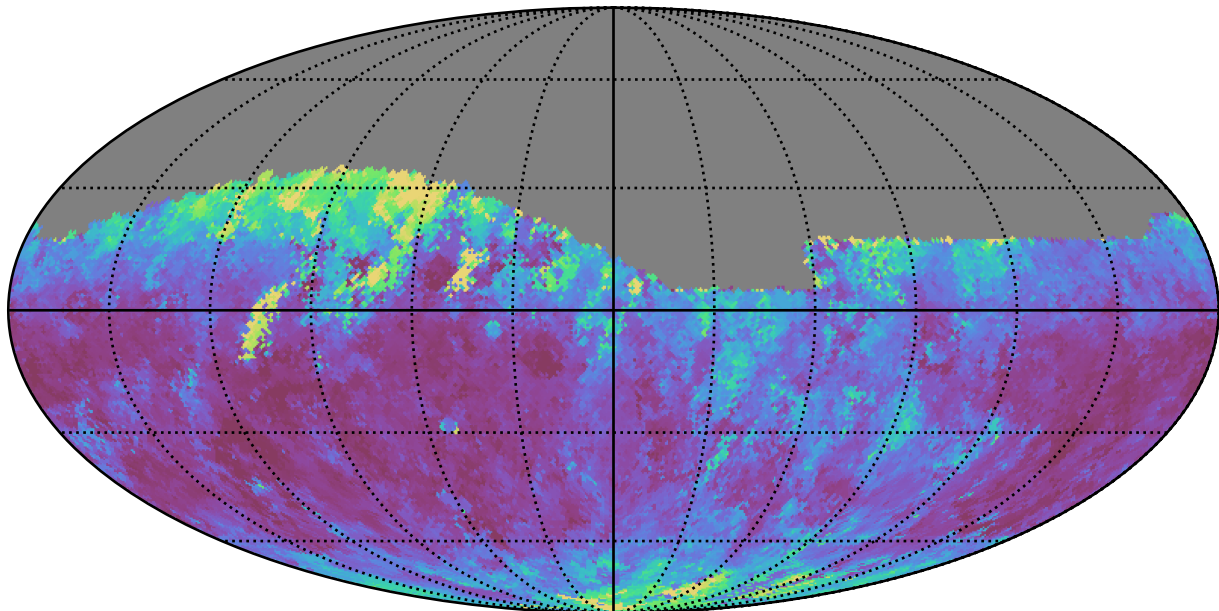
too_elab_r32_d3_gz_v3.4_10yrs Yr 1 r band: Median seeingGeom
