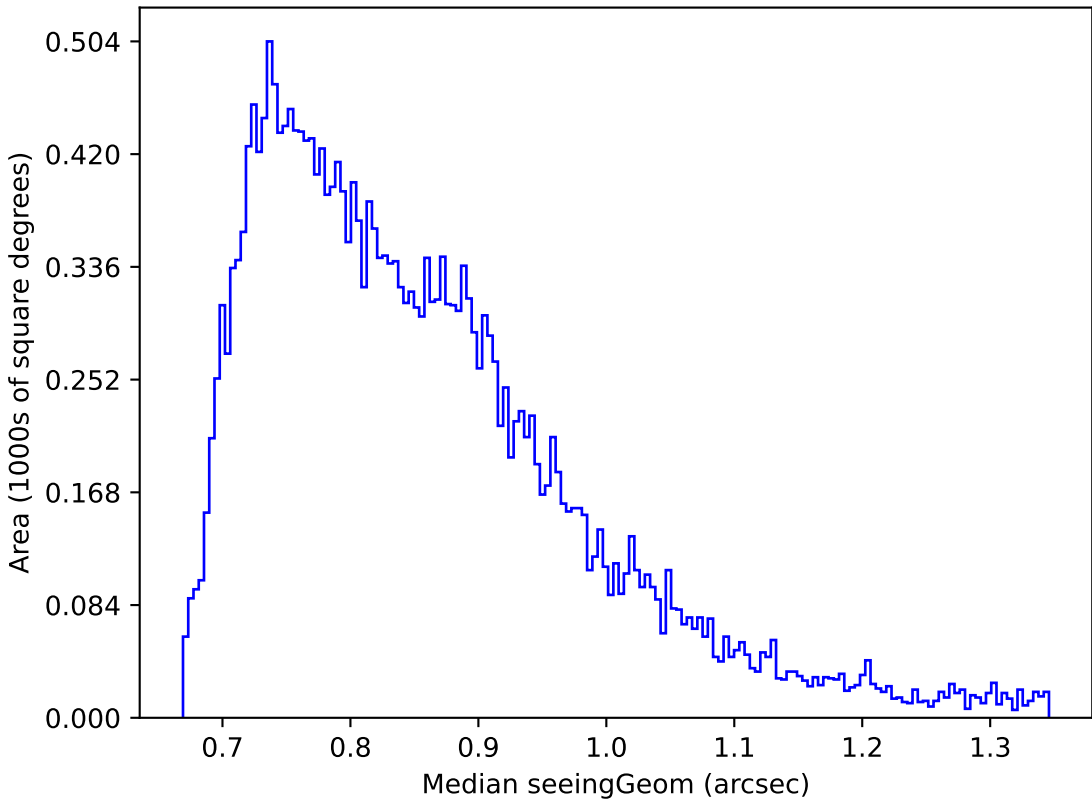
too_elab_r32_d3_gz_v3.4_10yrs Yr 1 r band: Median seeingGeom
