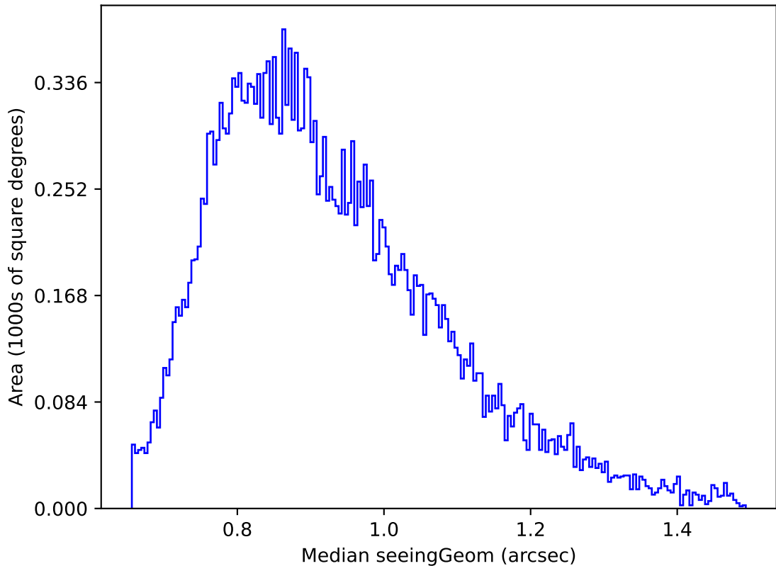
too_elab_r32_d3_gz_v3.4_10yrs Yr 1 g band: Median seeingGeom
