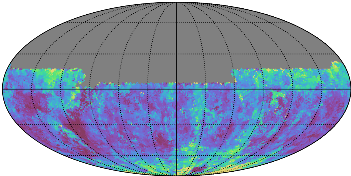
too_elab_r32_d3_gz_v3.4_10yrs Yr 1 y band: Median seeingEff
