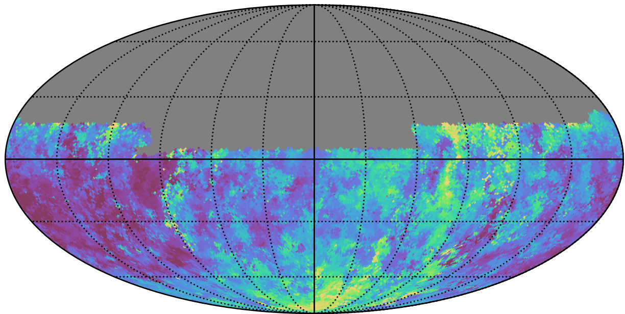
too_elab_r32_d3_gz_v3.4_10yrs Yr 1 u band: Median seeingEff
