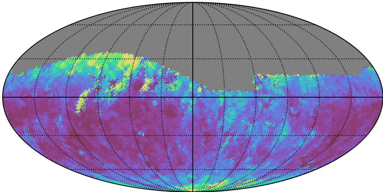
too_elab_r32_d3_gz_v3.4_10yrs Yr 1 r band: Median seeingEff
