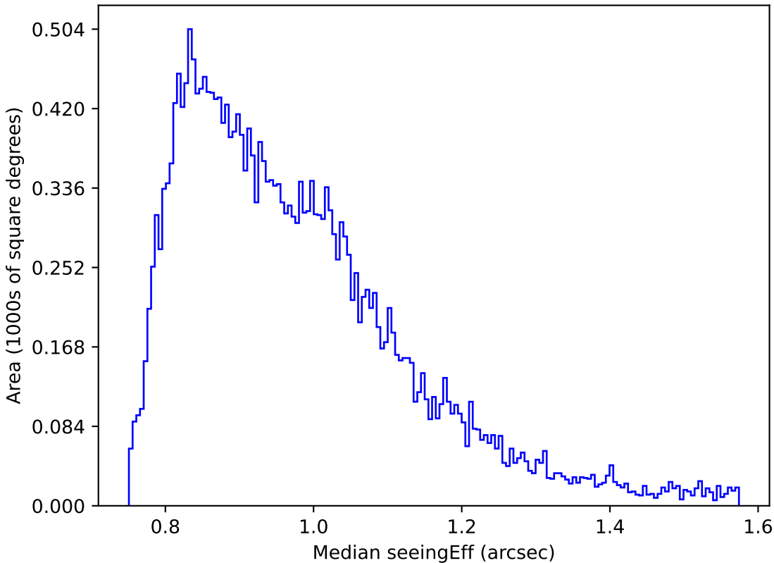
too_elab_r32_d3_gz_v3.4_10yrs Yr 1 r band: Median seeingEff
