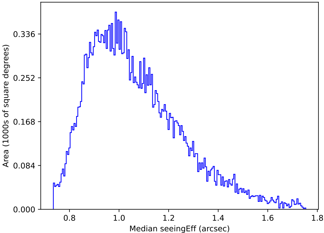
too_elab_r32_d3_gz_v3.4_10yrs Yr 1 g band: Median seeingEff
