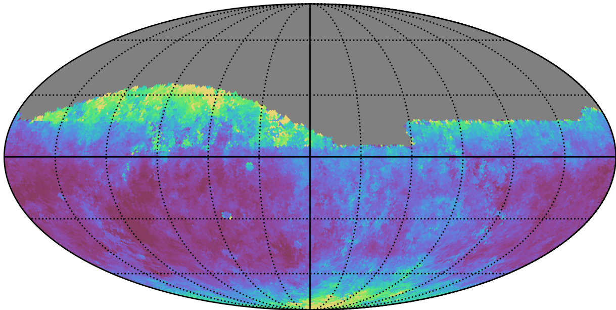
too_elab_r32_d3_gz_v3.4_10yrs Yr 1 all bands: Median seeingEff
