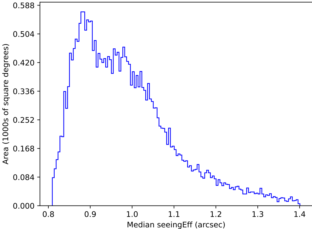
too_elab_r32_d3_gz_v3.4_10yrs Yr 1 all bands: Median seeingEff
