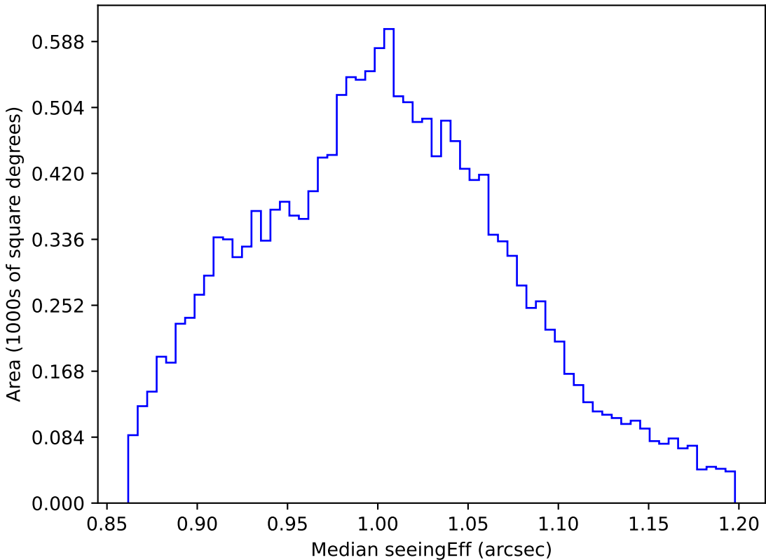
too_elab_r32_d3_gz_v3.4_10yrs WFD z band: Median seeingEff
