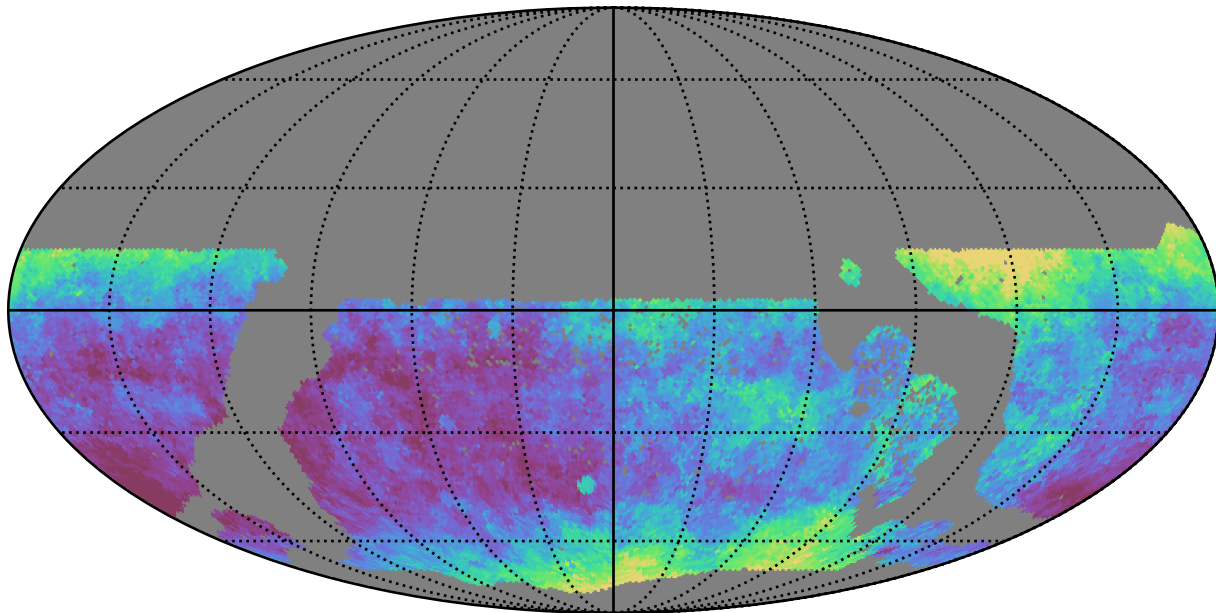
too_elab_r32_d3_gz_v3.4_10yrs WFD y band: Median seeingEff
