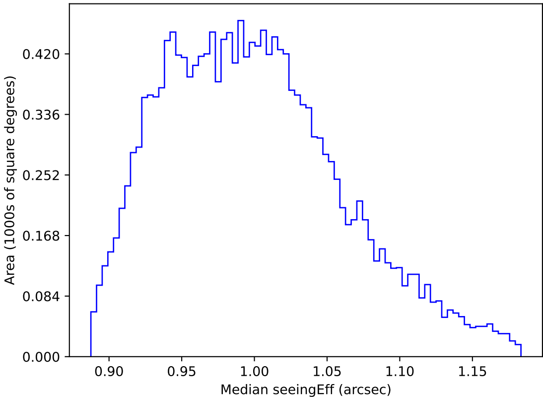
too_elab_r32_d3_gz_v3.4_10yrs WFD y band: Median seeingEff
