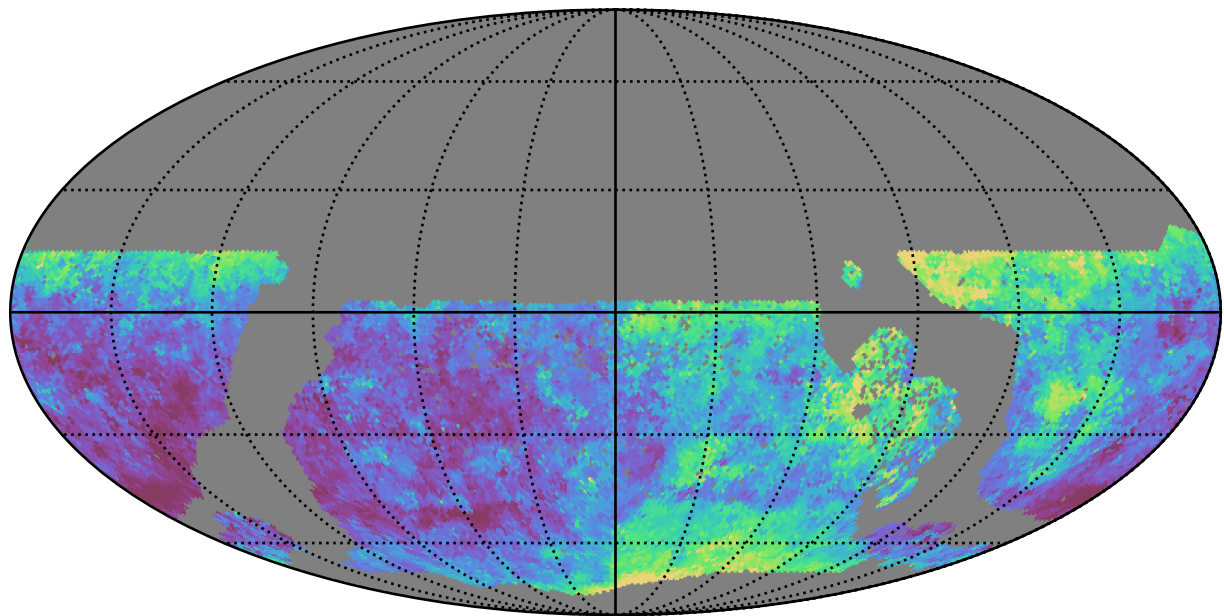
too_elab_r32_d3_gz_v3.4_10yrs WFD u band: Median seeingEff
