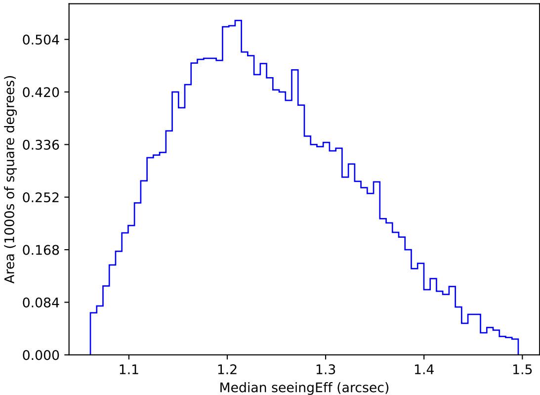
too_elab_r32_d3_gz_v3.4_10yrs WFD u band: Median seeingEff
