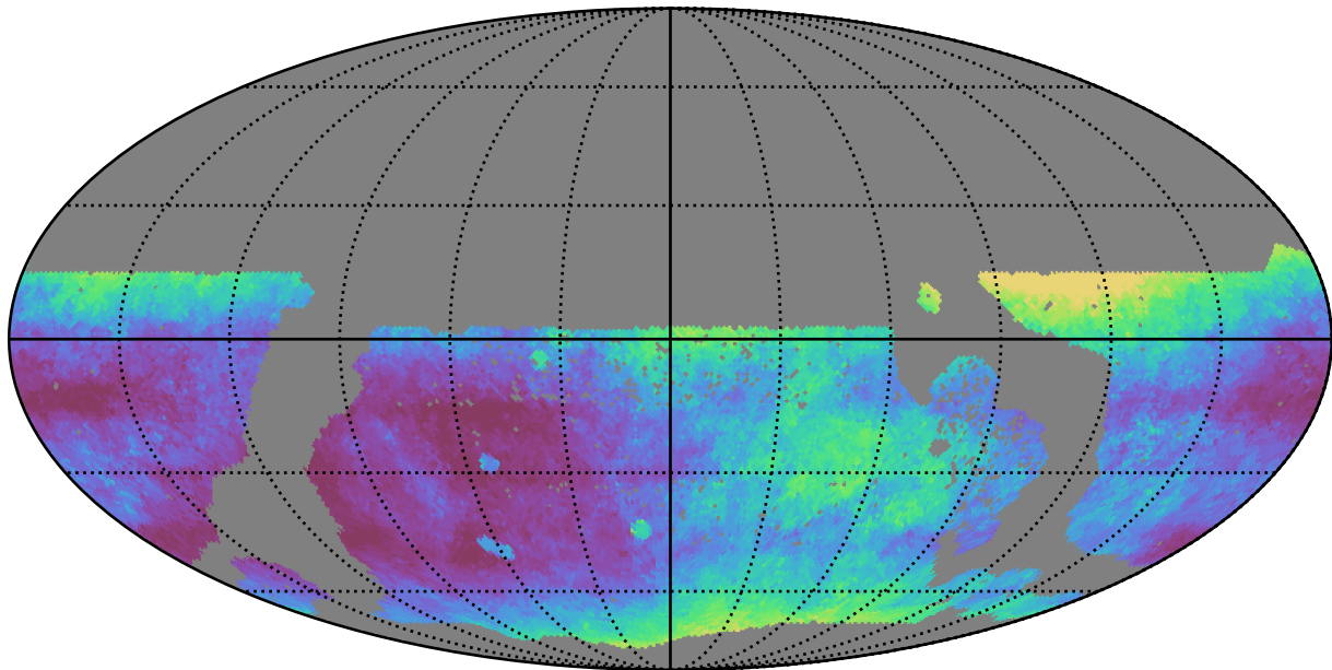
too_elab_r32_d3_gz_v3.4_10yrs WFD r band: Median seeingEff
