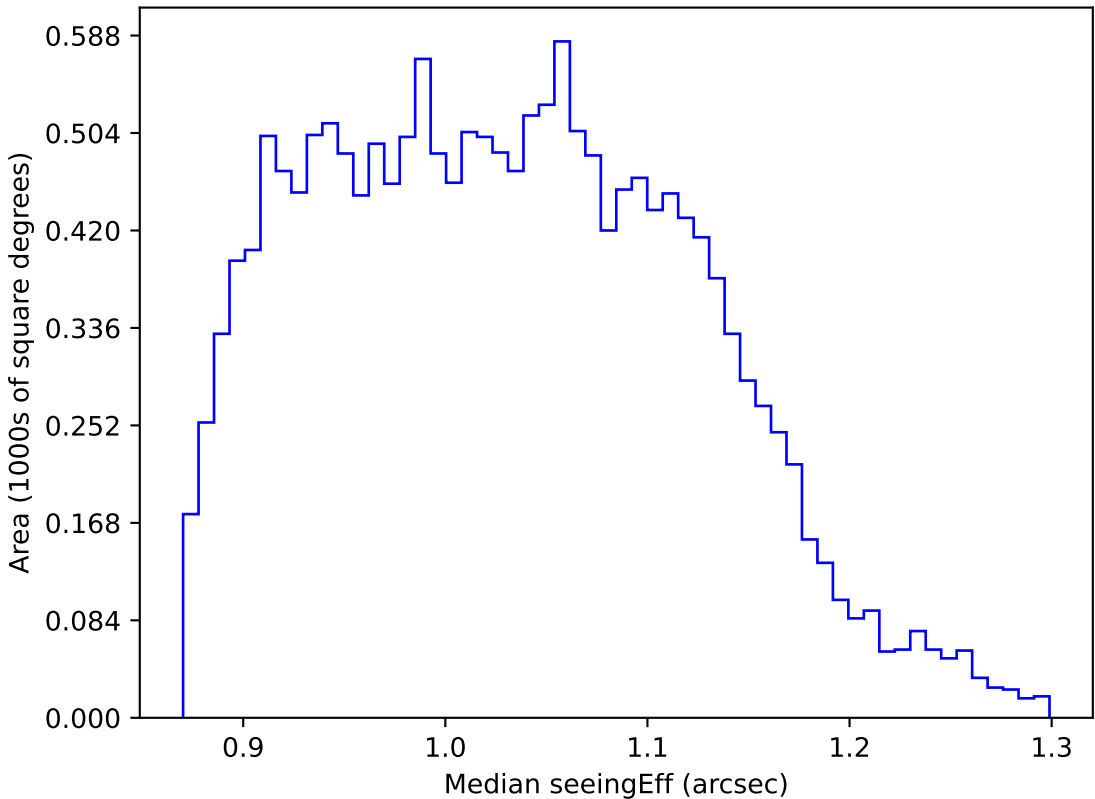
too_elab_r32_d3_gz_v3.4_10yrs WFD r band: Median seeingEff
