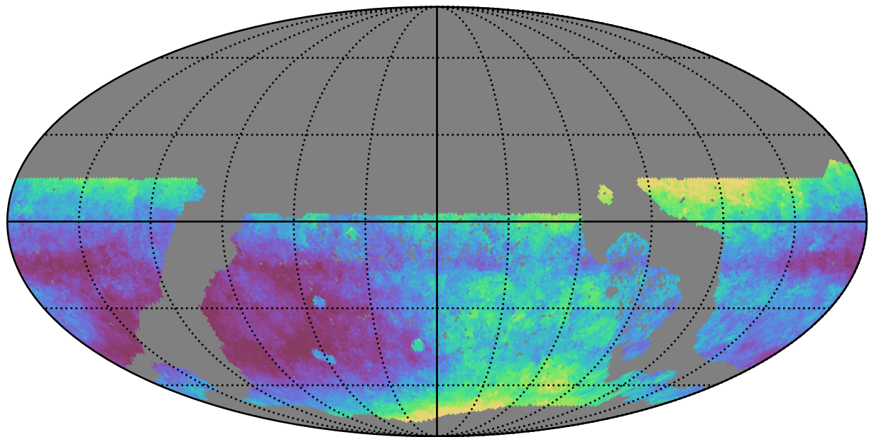
too_elab_r32_d3_gz_v3.4_10yrs WFD i band: Median seeingEff
