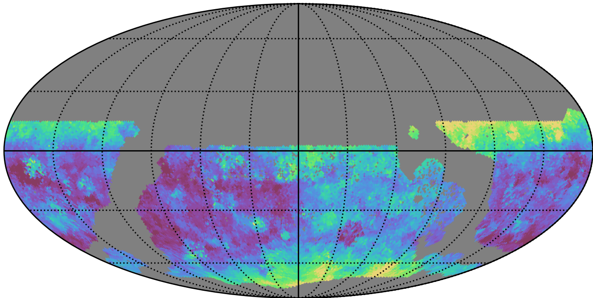
too_elab_r32_d3_gz_v3.4_10yrs WFD g band: Median seeingEff
