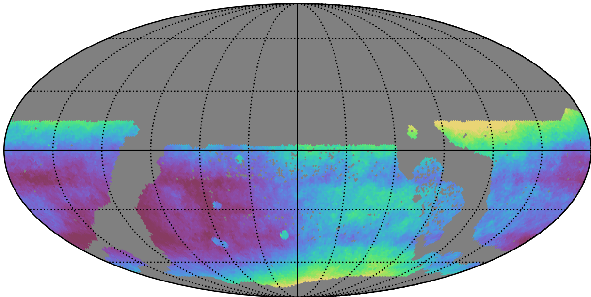
too_elab_r32_d3_gz_v3.4_10yrs WFD all bands: Median seeingEff
