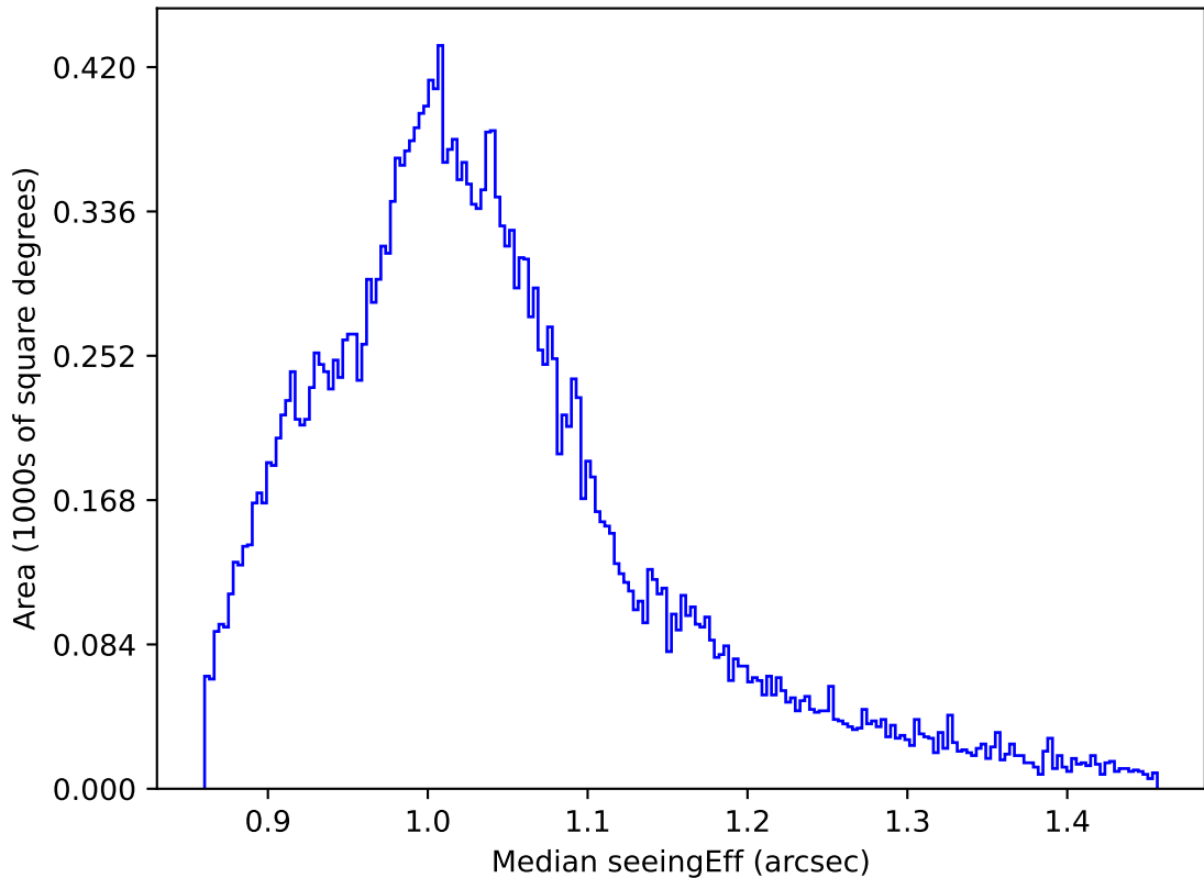
too_elab_r32_d3_gz_v3.4_10yrs All sky z band: Median seeingEff
