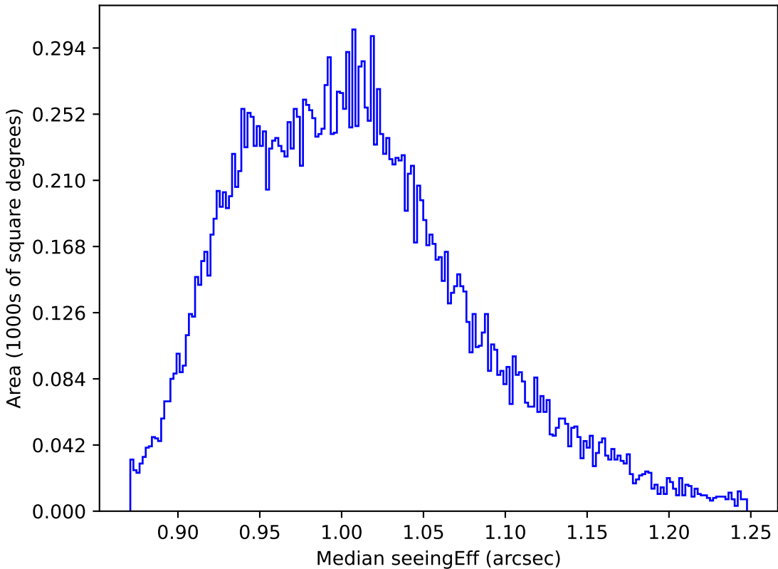
too_elab_r32_d3_gz_v3.4_10yrs All sky y band: Median seeingEff
