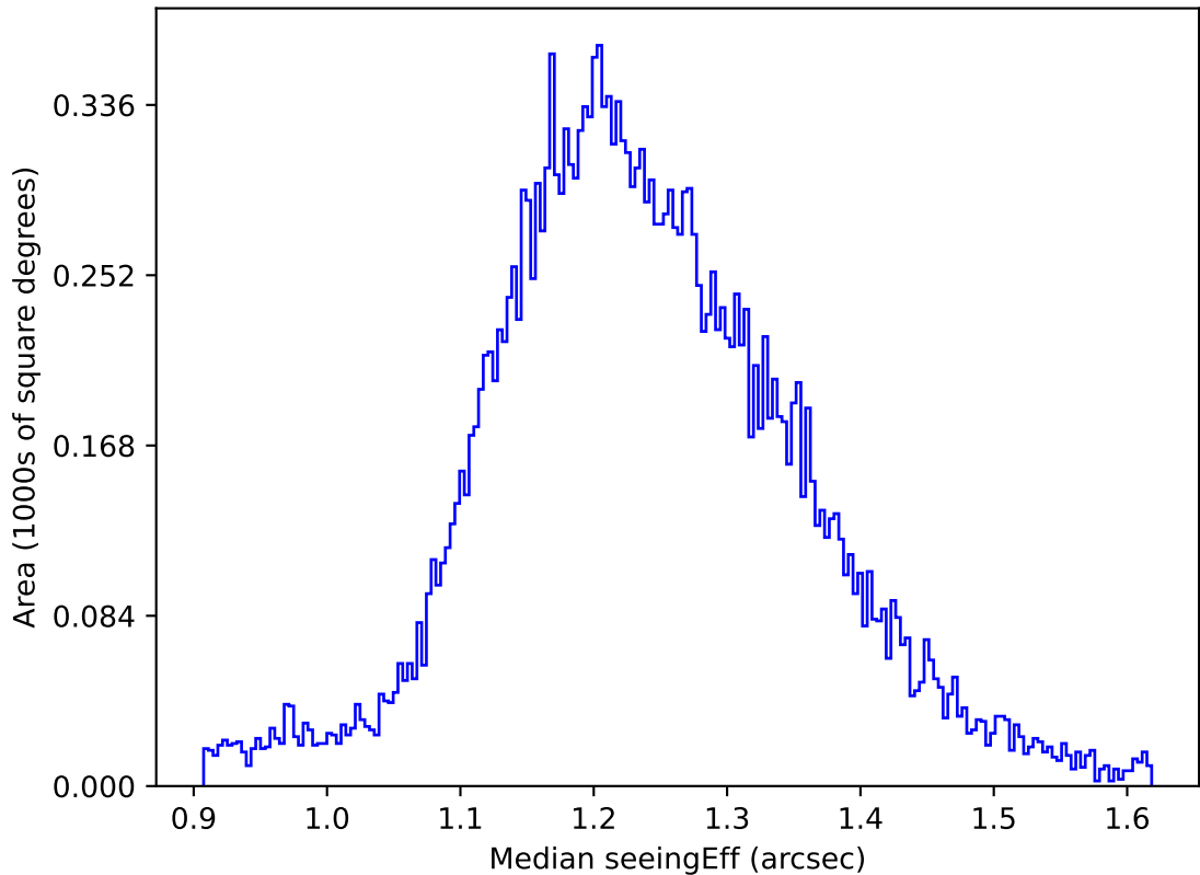
too_elab_r32_d3_gz_v3.4_10yrs All sky u band: Median seeingEff
