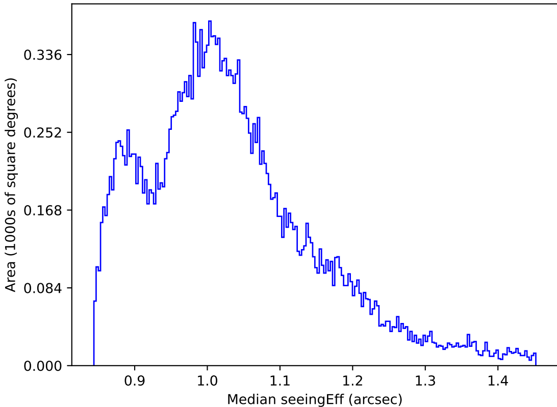
too_elab_r32_d3_gz_v3.4_10yrs All sky i band: Median seeingEff
