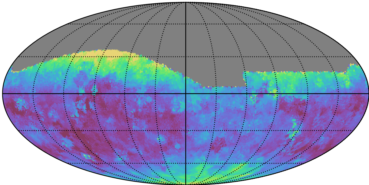
too_elab_r32_d3_gz_v3.4_10yrs All sky g band: Median seeingEff
