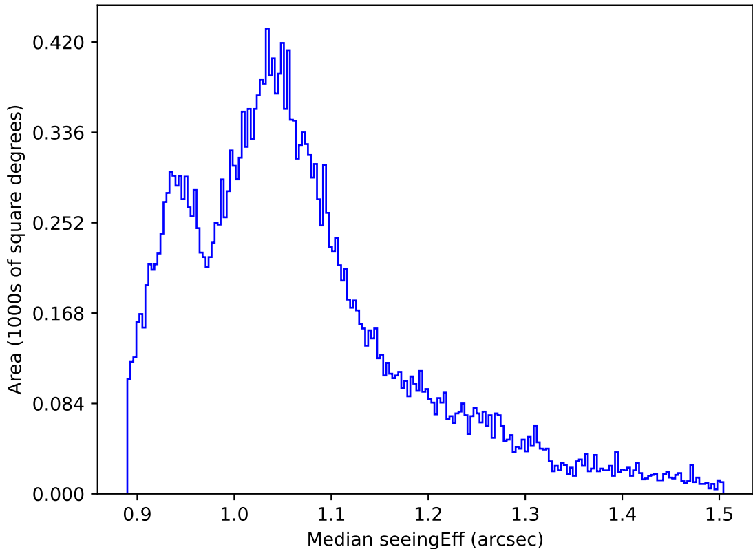
too_elab_r32_d3_gz_v3.4_10yrs All sky all bands: Median seeingEff
