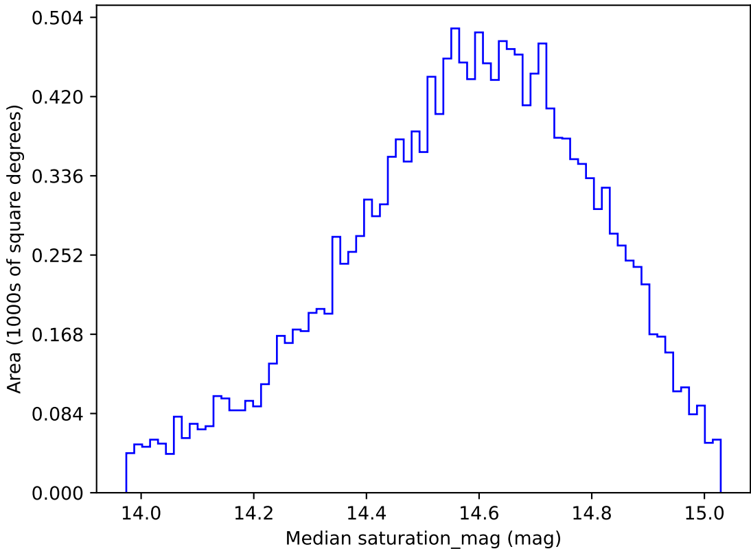
too_elab_r32_d3_gz_v3.4_10yrs WFD g band: Median saturation_mag
