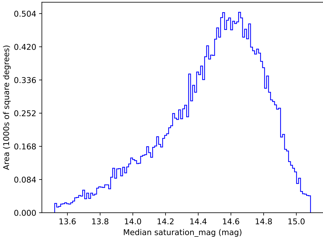
too_elab_r32_d3_gz_v3.4_10yrs All sky g band: Median saturation_mag
