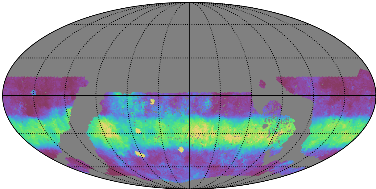
too_elab_r32_d3_gz_v3.4_10yrs WFD z band: Median normairmass
