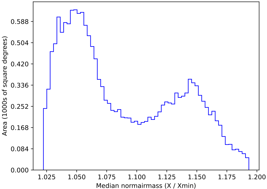
too_elab_r32_d3_gz_v3.4_10yrs WFD z band: Median normairmass
