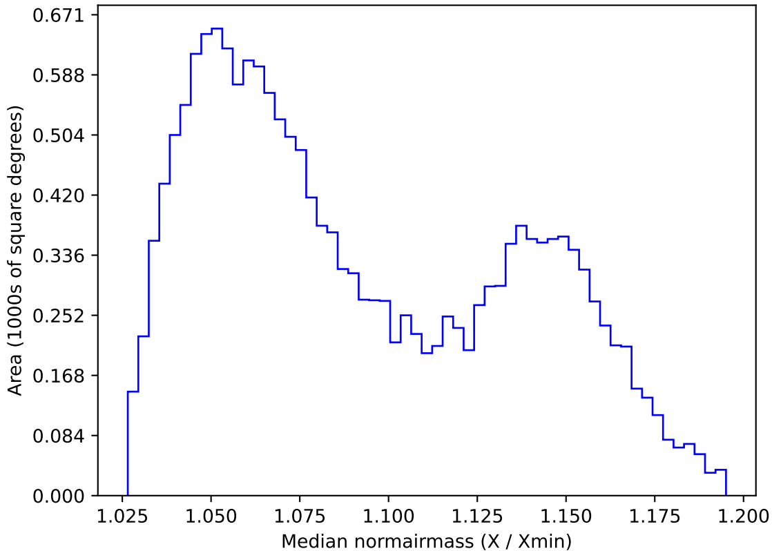
too_elab_r32_d3_gz_v3.4_10yrs WFD y band: Median normairmass
